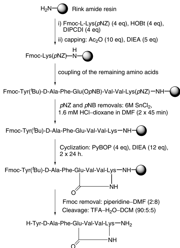
Scheme 2. Solid-phase synthesis of the deltorphin cyclic analog, H-Tyr-D-Ala-Phe-Glu(&)-Val-Val-Lys(&)-NH 2 .
