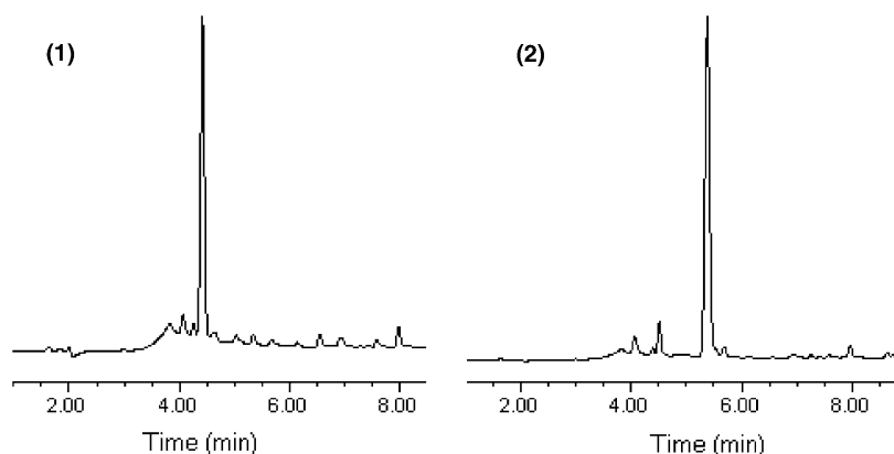
Figure 2. HPLC chromatograms of \text{H-Orn(Phe)-Ala-NH}_2 ( 1 ) and \text{H-Phe-Orn(Phe)-Ala-NH}_2 ( 2 ).
