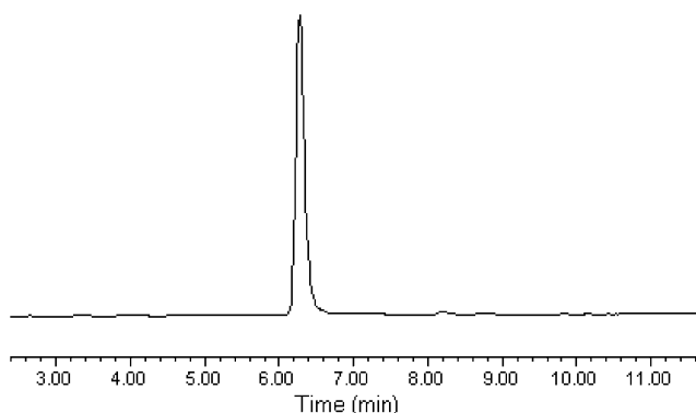
Figure 3. HPLC chromatogram of the cyclic deltorphin analog H-Tyr-D-Ala-Phe-Glu(&)-Val-Val-Lys(&)-NH 2 .
